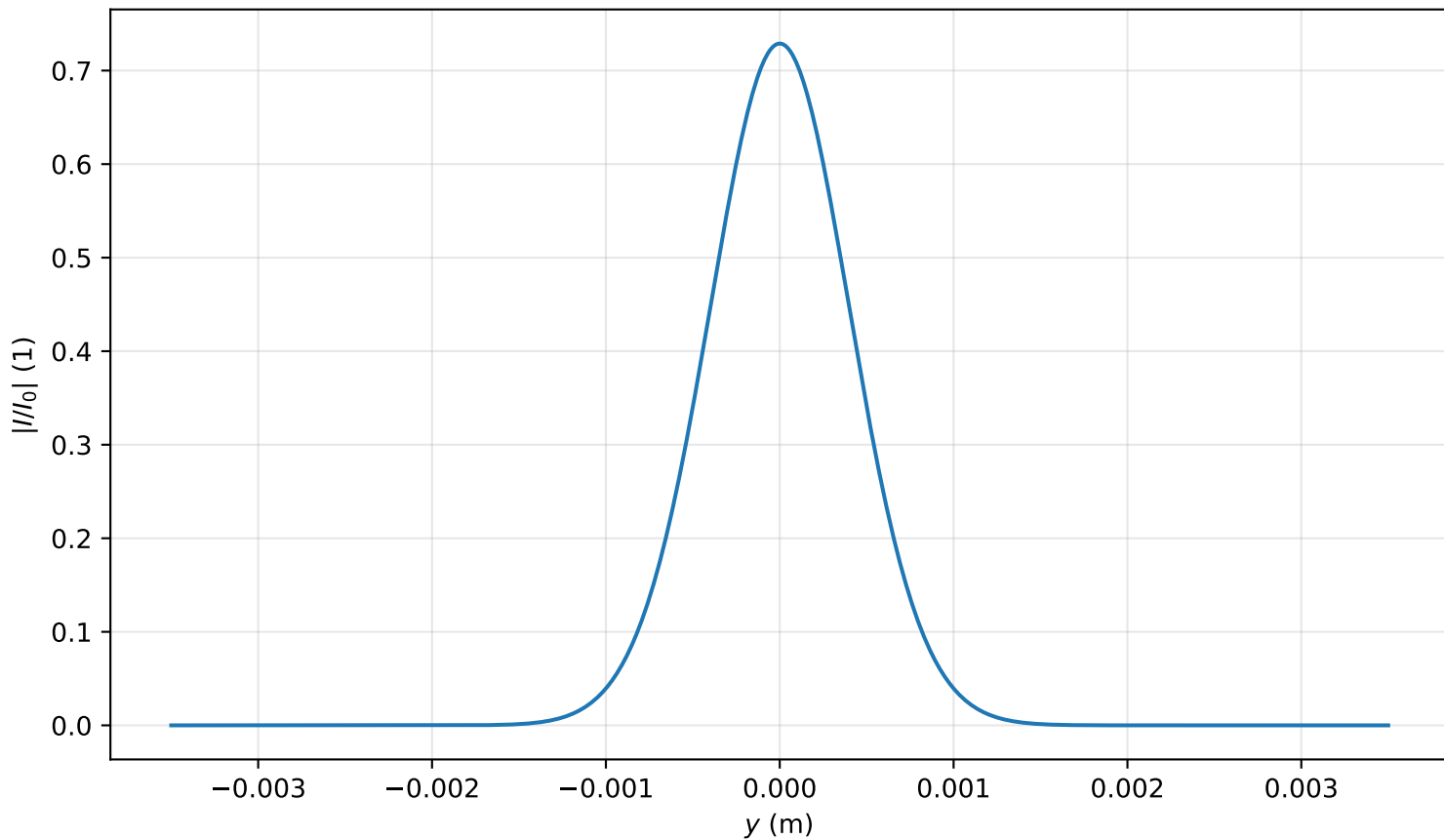
Intensity profile I(x=0, y, z=1.353)/I_0 , \text{Pin}=0.1\text{Pcr} , artificial time
